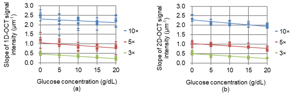
Fig. 2. Slope of OCT signal intensity vs. depth plotted against the glucose concentration in the phantom: (a) 1D and (b) 2D scan measurements. Each line indicates the linear regression.
