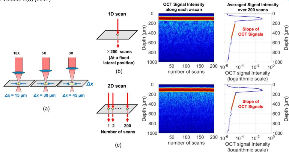
Fig. 1. Measurement areas using LM-OCT system equipped with lenses of 10×, 5×, and 3× (a) and typical examples of the changes in OCT signal intensities as a function of the sample depth obtained by 1D (b) and 2D (c) scans with an objective lens of 10×. The values of the logarithm of the signal intensity shown with a pseudo color in the middle figures are shown in the horizontal axes in the right figures.
