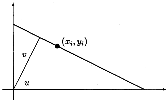
図 1: u-v transformation.
