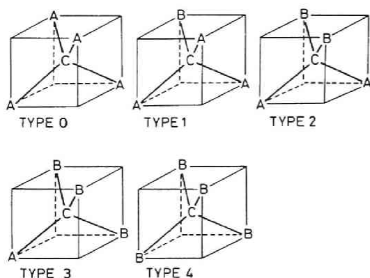
Fig.3-1 Tetrahedron cells in a ternary alloy semiconductor A_{1-x}^{III}B_x^{III}C^V or C_{1-x}^{III}A_x^V B_x^V .
