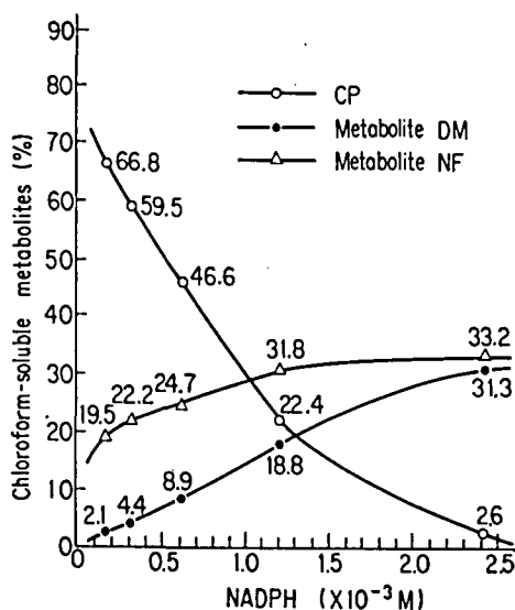
Fig. 1. Degradation of ^{14}\text{C} -CP-HCl by the concentration of NADPH at rat-liver microsomes. Open circle represents unchanged CP [ N -(4-chloro- o -tolyl)- N' , N' -dimethylformamidine]; close circle, metabolite DM [ N -(4-chloro- o -tolyl)- N' -methylformamidine], and also triangle circle metabolite NF [ N -formyl-4-chloro- o -toluidine]. Incubation time was 60 minutes.
