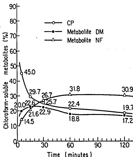
Fig. 2. The relationship between the reaction time and the amounts of metabolites on the degradation of ^{14}\text{C} -CP-HCl by rat-liver microsomes + NADPH-system. Circles were identical to those described in Fig.1.
