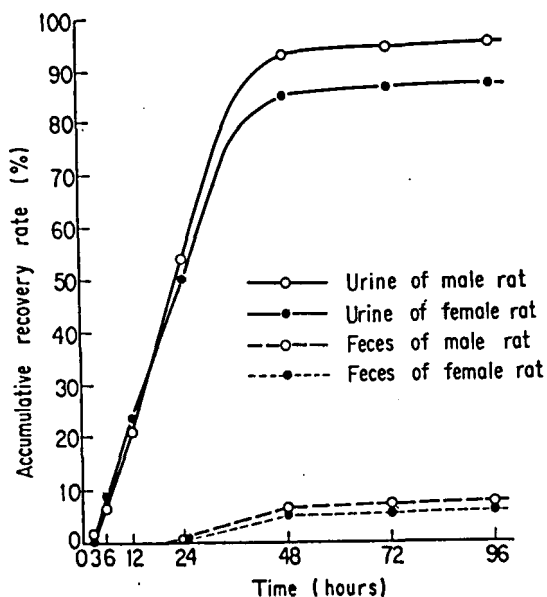
Fig. 3. Accumulative recovery rate of radioactive substances into urine and feces of 2 rat after oral administration of ^{14}\text{C} -CP-HCl.
