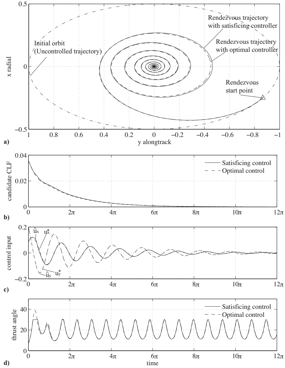
Figure 5.12: a) Rendezvous trajectories with satisficing and optimal control, b) Profiles in candidate CLF, c) input \mathbf{u} , and d) thrust angle \delta . Parameter setting q_r = q = 0.1 , q_v = 0 , \lambda_\alpha = \sqrt{0.9q} , \varphi_0 = 120^\circ , \alpha = 30^\circ .
