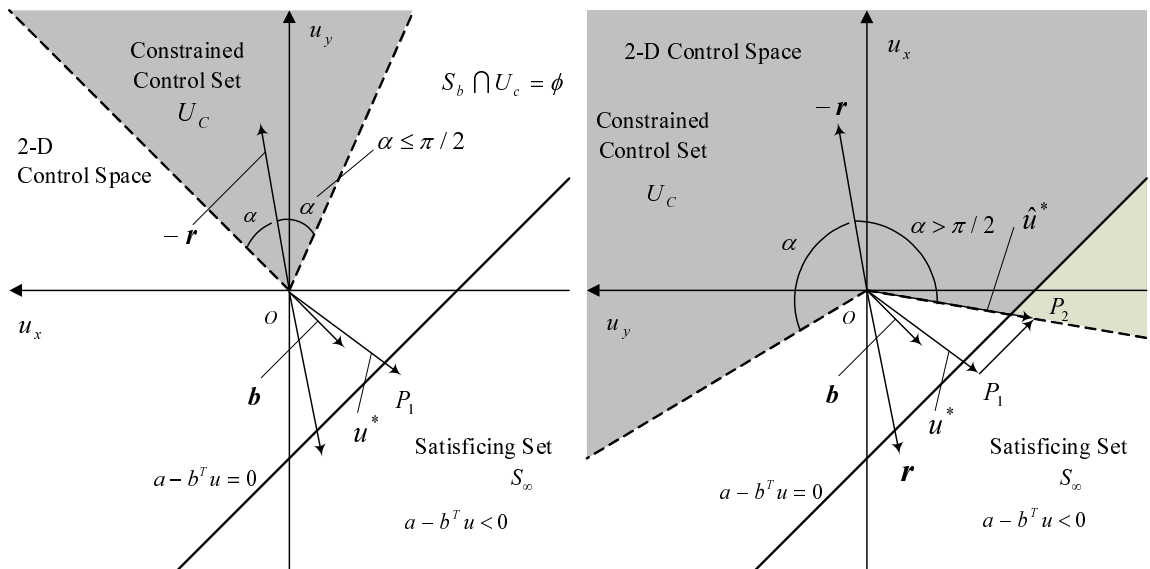
Figure 5.5: Performing projection onto the restricted area.
