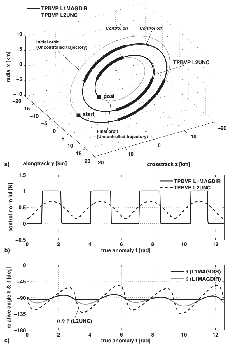
Figure 3.10: Solutions for (\mathcal{P}^{\epsilon}_{md1}) . a) 3D-trajectory, b) profiles in \|u^{\epsilon}_{mdj}\| , and c) \theta and \beta .
