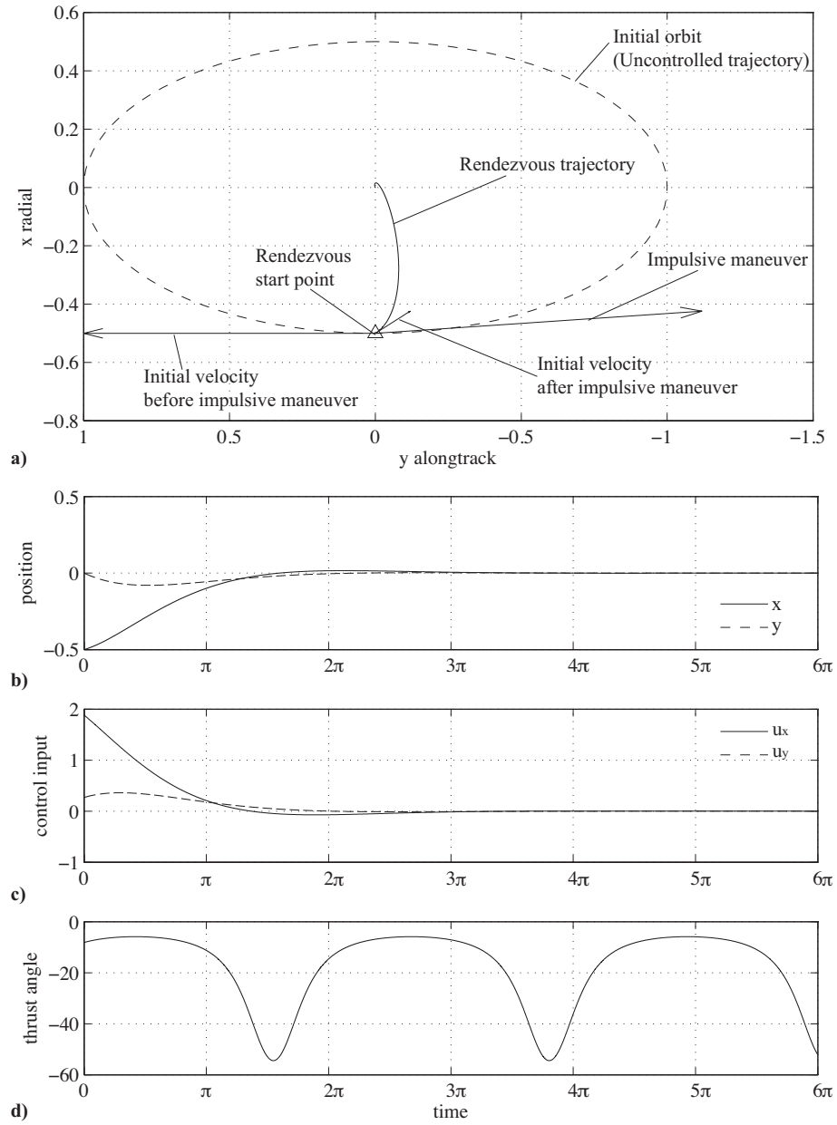
Figure 5.10: a) Rendezvous trajectory leaving \lambda_2 , \bar{\lambda}_2 mode, b) Profiles in position \mathbf{r} , c) input \mathbf{u} , and d) thrust angle \delta [°]. Parameter setting q_r = q = 10 , q_v = 0 , \lambda_\alpha = \sqrt{0.9q} , \varphi_0 = 180^\circ .
