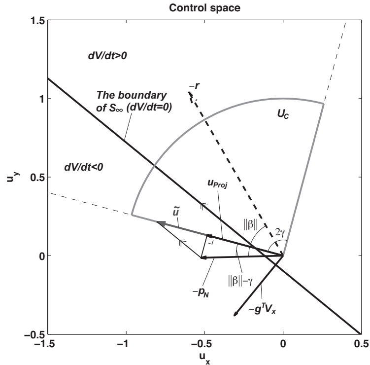
Figure 6.2: The difference in projection between \tilde{\mathbf{u}} and \mathbf{u}_{Proj} .
