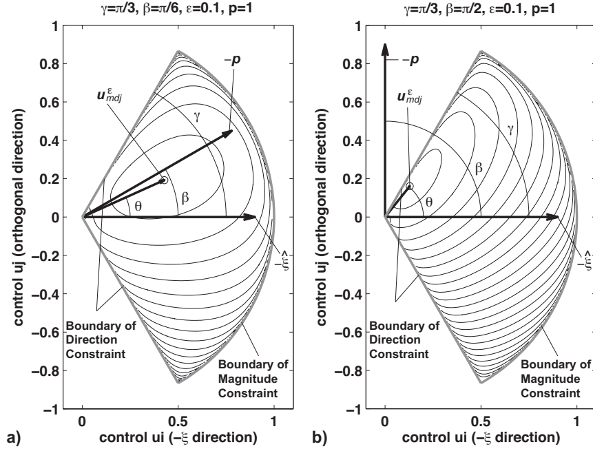
Figure 3.3: Illustration of the Hamiltonian contour in the 2-D control frame (i, j) . a) \beta < \gamma , b) \beta > \gamma .
