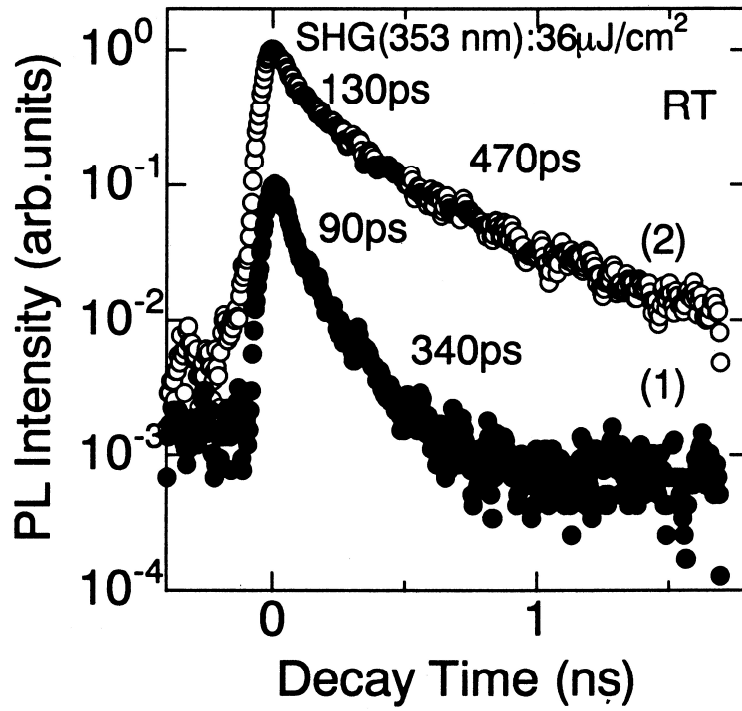
Fig. 3.32. Photoluminescence decay spectra of sample (a) (1) at a seed region (TDD = 10 9 cm -2 ) and (2) at a wing region (TDD = 10 6 cm -2 ).
