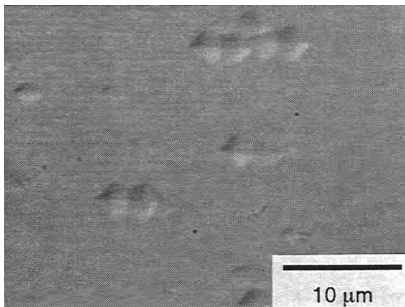
Fig. 3.18. Nomarski interference micrograph of a ZnMgSSe:N film grown CSMBE at 280°C with 2.6 \mu\text{m/h} .
