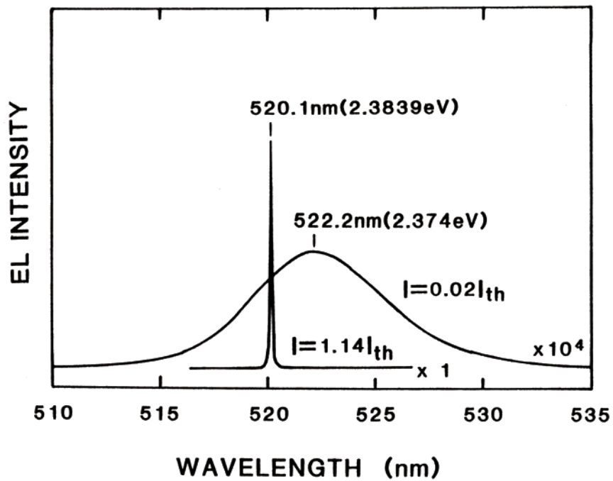
Fig. 1.3. Spontaneous and stimulated emission spectra for a \text{Zn}_{0.7}\text{Cd}_{0.3}\text{Se} SQW LD under pulsed current injection at 77 K.
