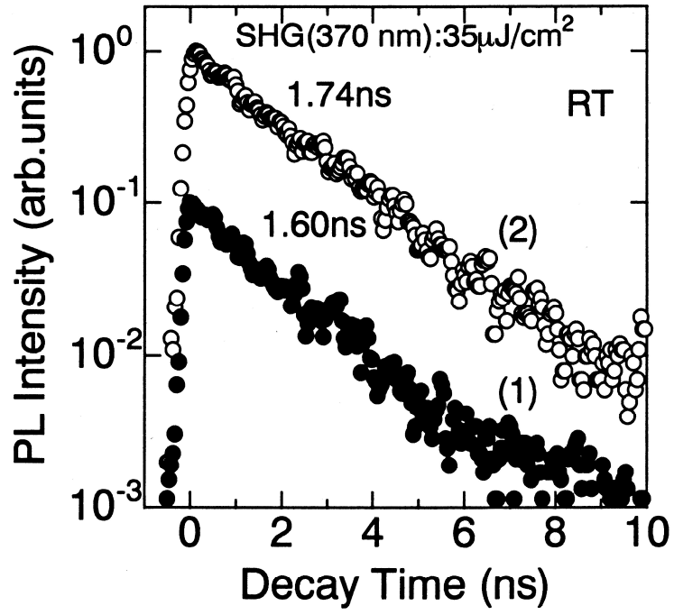
Fig. 3.33. Photoluminescence decay spectra of sample (b) (1) at a seed region ( TDD = 10^9 \text{ cm}^{-2} ) and (2) at a wing region ( TDD = 10^6 \text{ cm}^{-2} ).
