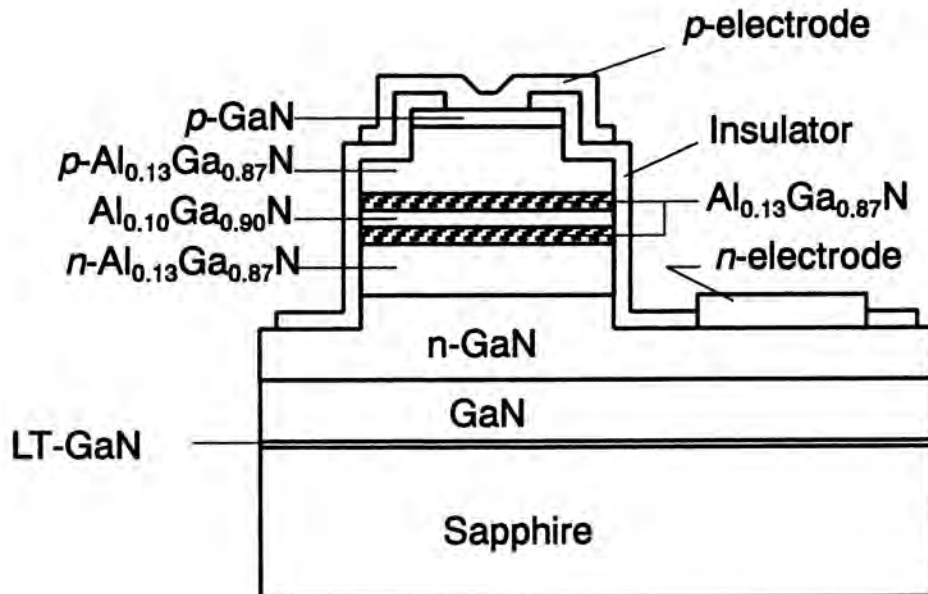
Fig. 2.11. Schematic of Al 0.13 Ga 0.87 N/Al 0.10 Ga 0.90 N ridge stripe BLDH structure.
