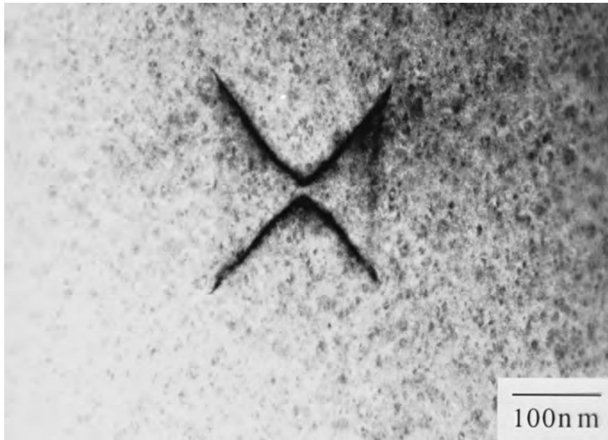
Fig. 3.4. Plan-view TEM showing a pair of stacking faults. The sample was thinned, i.e. the p-side layers were removed.
