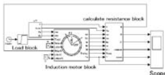
Fig. 2 Analysis code of HTS-ISM with MATLAB®/Simulink®
