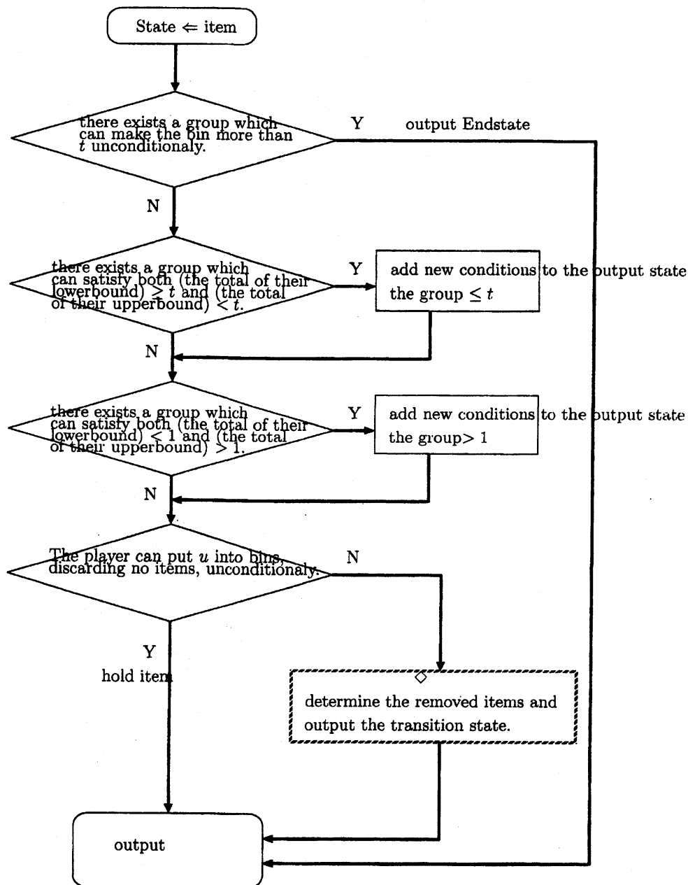
Figure 5: Flow chart of an algorithm \mathcal{A}
