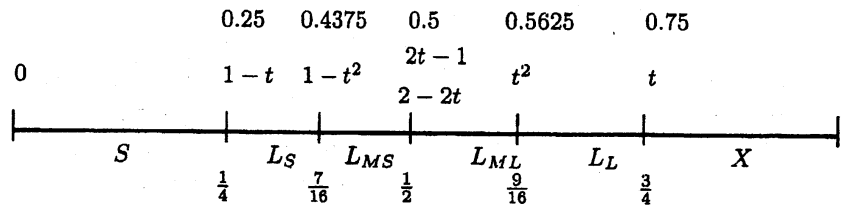
Figure 3: Classification of the items according to their sizes.
