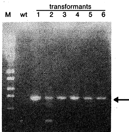
M: \lambda -EcoT141 digest
