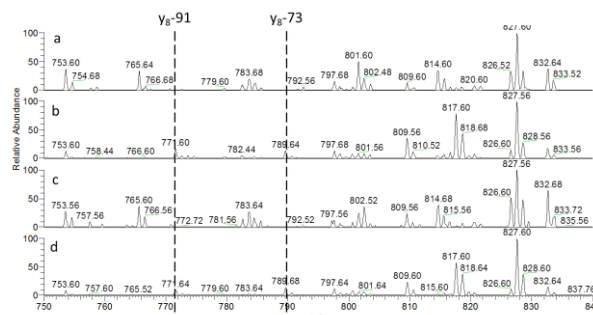
Fig. 1 Second generation product ion spectra of four isomeric Asp residues in \alpha AT6 synthetic peptides; a) \alpha AT6- L\alpha , b) \alpha AT6- L\beta , c) \alpha AT6- D\alpha and d) \alpha AT6- D\beta .
