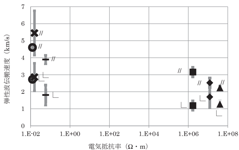
図2 木炭の電気抵抗率と硬度（上）および弾性波伝搬速度（下）との関係 Figure 2. Relationships between hardness (upper), speed of elastic wave (lower) and electric resistivity
