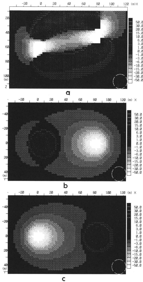
Fig. 2 Examples of the three-dimensional sensitivity analysis of electrical method. (a) Sensitivity distribution at the vertical section with the electrodes for CC(subsurface, borehole DH-1)PP(subsurface, borehole DH-2) solid array system, (b) Sensitivity distribution at the horizontal section in the depth of 40 m for the same electrode array as the case shown in Figure 2a, (c) Sensitivity distribution at the horizontal section in the depth of 60 m for the same electrode array as the case shown in Figure 2a.
