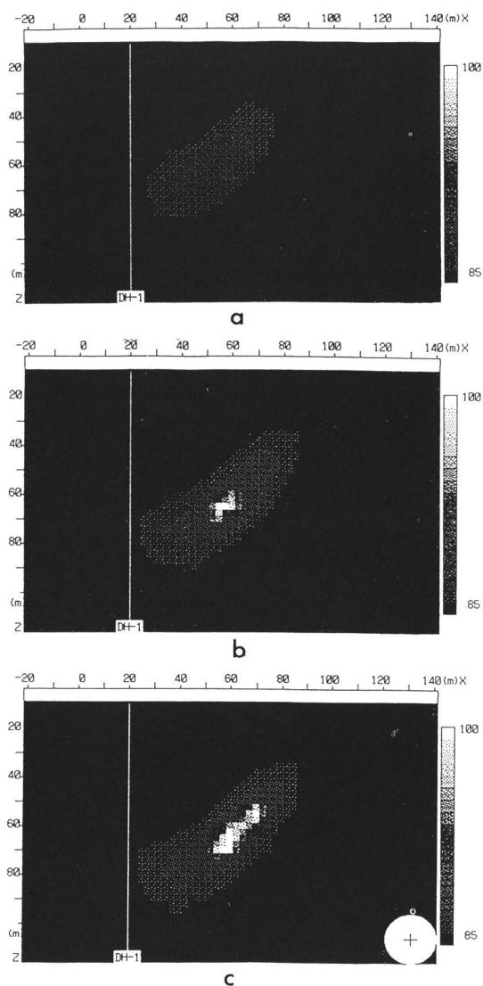
Fig. 9 Three-dimensional computerized vertical sections reconstructed by the differential sensitivity distribution technique for the same solid array system as the case shown in Figure 7.
