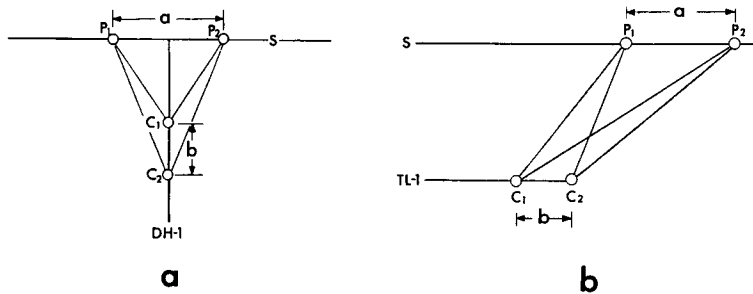
Fig. 3 Examples of differential solid electrode arrays.
