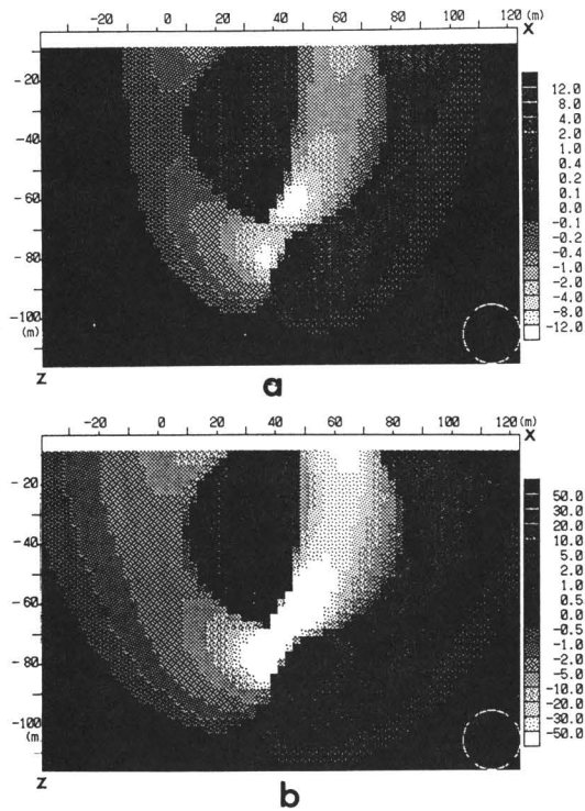
Fig. 5 Examples of the three-dimensional extended differential sensitivity analysis of electrical method.
