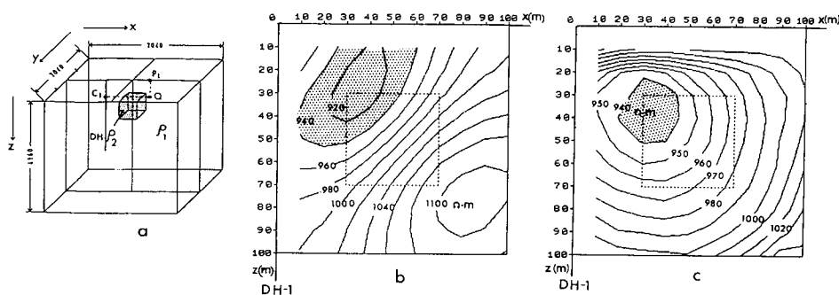
Fig. 1 An example of three-dimensional modeling. 55)
