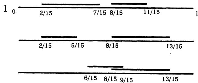
図5: G_{\frac{1}{3}}(\frac{1}{3}, \frac{1}{5}, \frac{1}{5})
