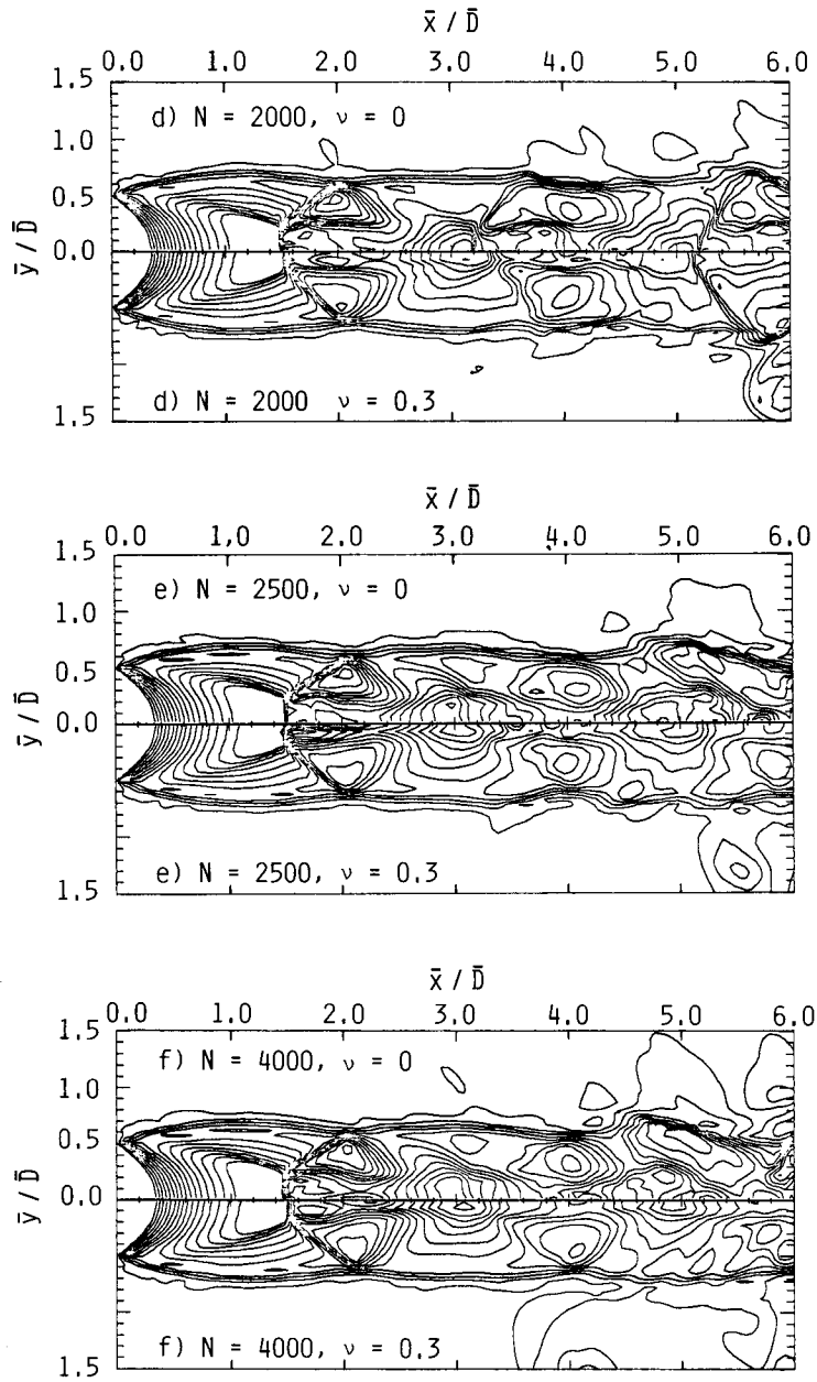
Fig. 6 Comparison of density contour of two-phase mixture flows with the corresponding dust-free ones at several kinds of time steps.
