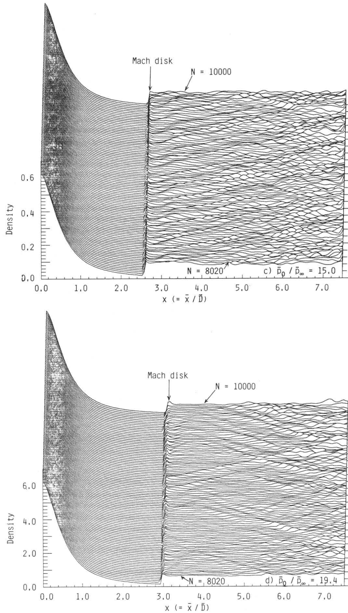
Fig. 4 Time history of density distribution along jet axis for 8020 \leq N \leq 10000 under the conditions corresponding to Fig. 3.
