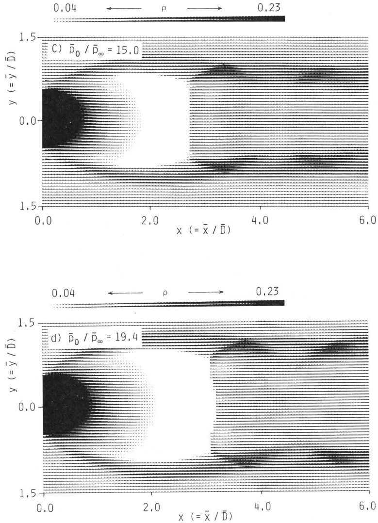
Fig. 3 Contours of constant density for underexpanded choked sonic jets of the four cases where \bar{p}_0 = 5.8 \times 10^5 Pa (a), \bar{p}_0 = 10.0 \times 10^5 Pa (b), \bar{p}_0 = 15 \times 10^5 Pa (c) and \bar{p}_0 = 19.4 \times 10^5 Pa (d).
