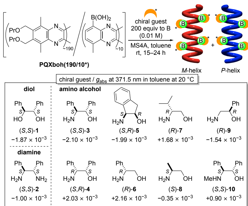
Scheme S4.
