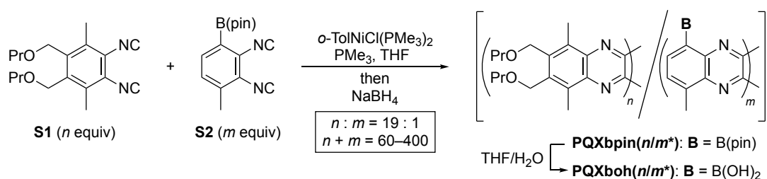
Scheme S1.
