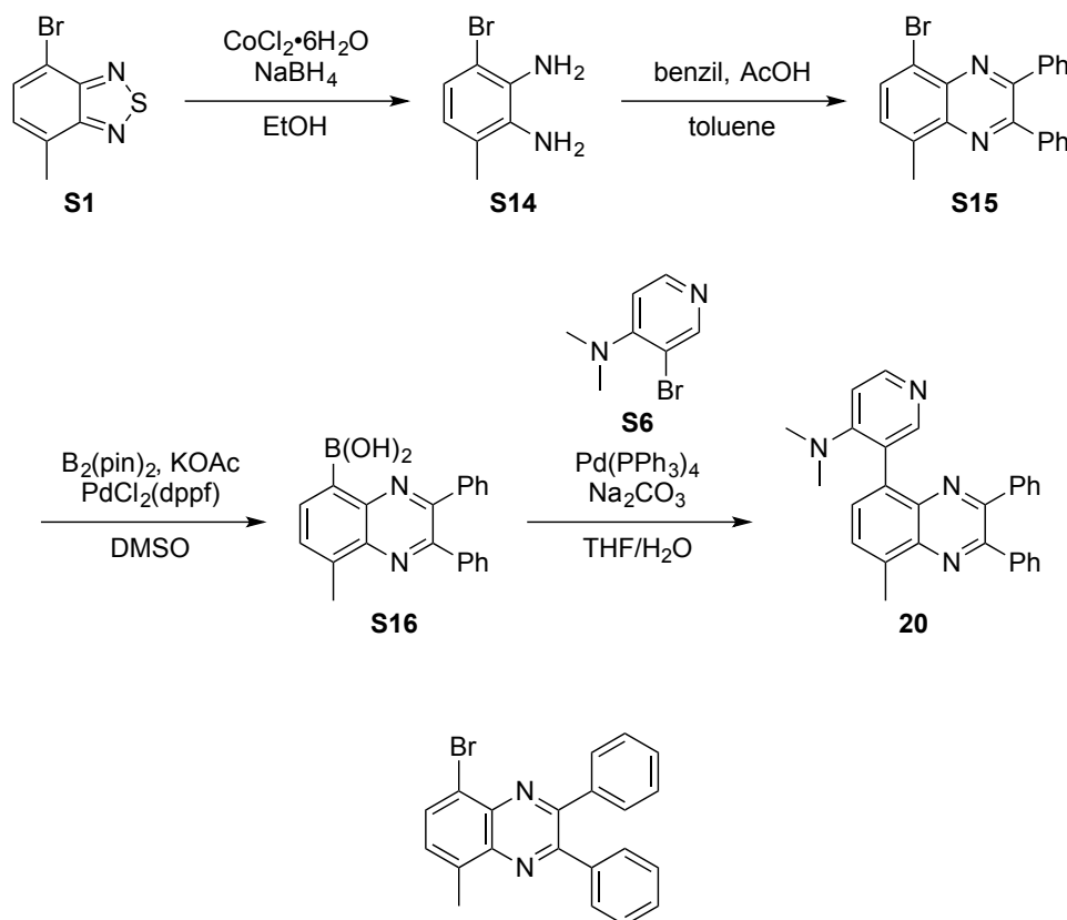
Scheme S3. Synthesis of Model Compound 20
