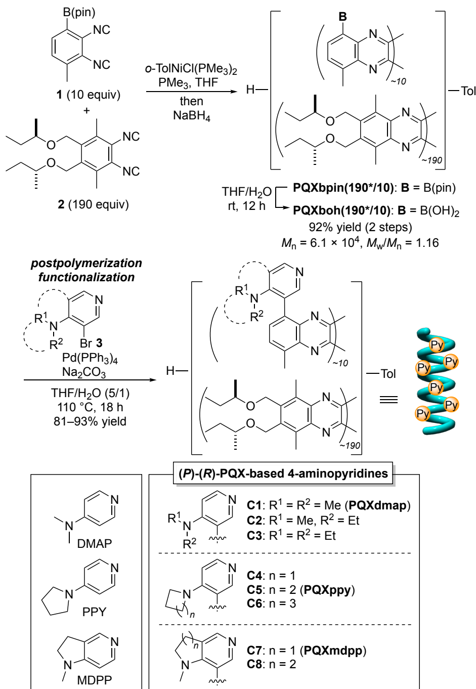
Scheme 2. Synthesis of Polyquinoxaline-based Helically Chiral Nucleophilic Catalysts
