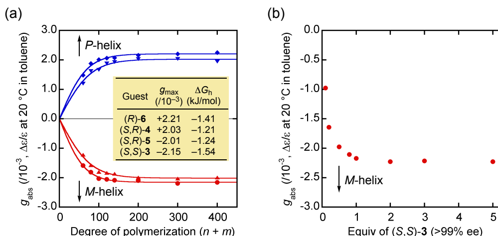
Figure 2. (a) Relationships between DP ( n+m ) and dissymmetry factor g of PQXboh ( n/m^* ) ( n/m = 19/1 ) at 371.5 nm in toluene at 20 °C: (S,S)-3 (red ●), (S,R)-4 (blue ▼), (S,R)-5 (red ▲), and (R)-6 (blue ◆). In the table insert, g_{\max} ( g values for pure helix) and \Delta G_h (helix stabilization energy per unit) calculated from curve fittings are shown. (b) Helical chirality induction of PQXboh (380/20 * ) with different equivalents (equiv) of (S,S)-3.
