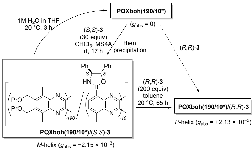
Scheme 1. Reversible Helical Chirality Induction of PQXboh with Chiral Amino Alcohol
