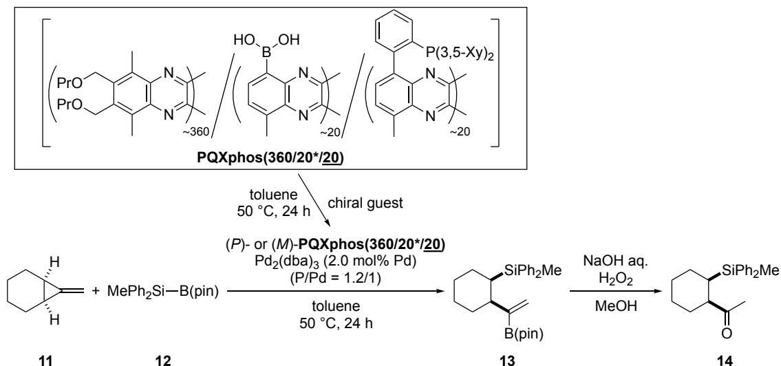
Scheme S5.
