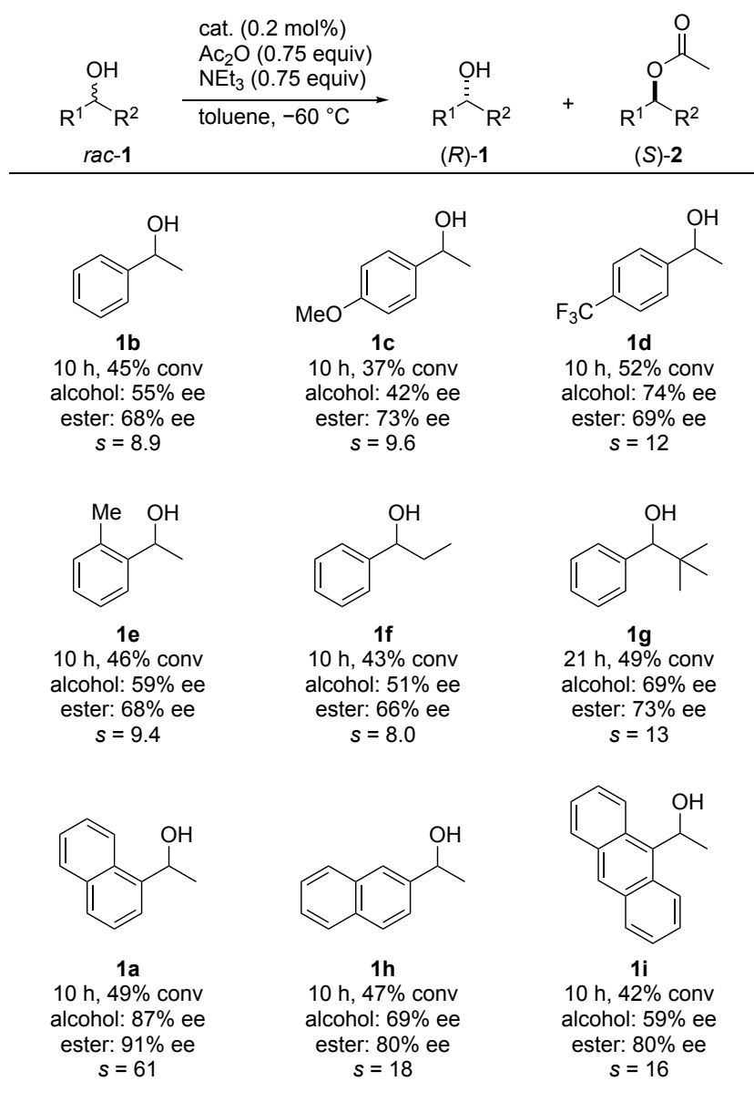
Scheme 1. Substrate Scope
