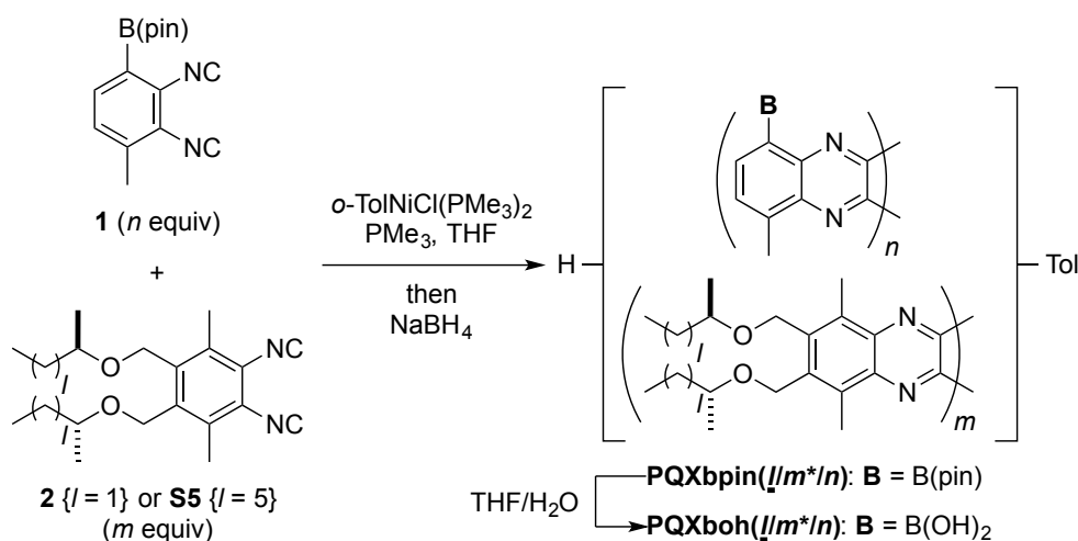
Scheme S2. Synthesis of ( P )-( R )-PQXboh( \underline{l}/m^*/n )
