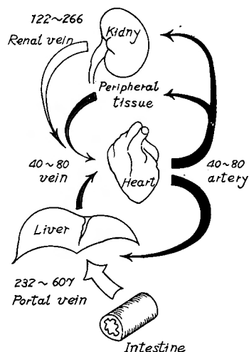
Fig. 3. Blood \text{NH}_3\text{-N} levels ( \gamma/\text{dl} ) in main blood vessels.
