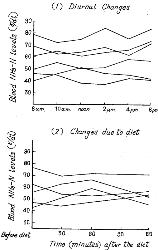
Fig. 2. Physiological changes in blood NH 3 -N levels.
