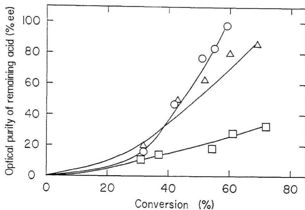
Fig. 3. Relationship between optical purity of the remaining acid and conversion ratio in esterification of 2-(4-chlorophenoxy)propanoic acid with different alcohols by lipase OF 360. (○), 1-Tetradecanol; (△), 1-hexanol; (□), ethanol.
