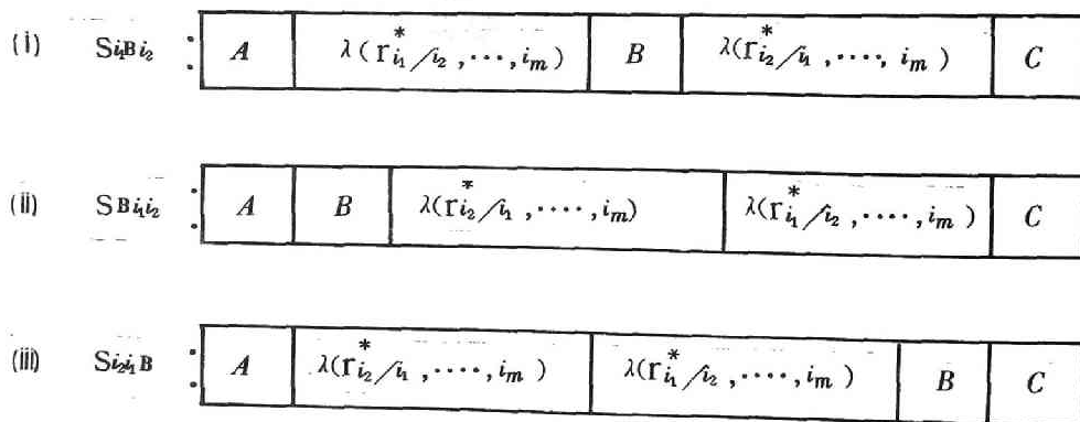
Fig. 2.10. Proof of Theorem 2.5.
