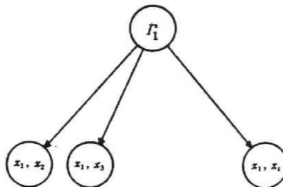
Fig.2.12. Illustration of a tree-like diagram.
