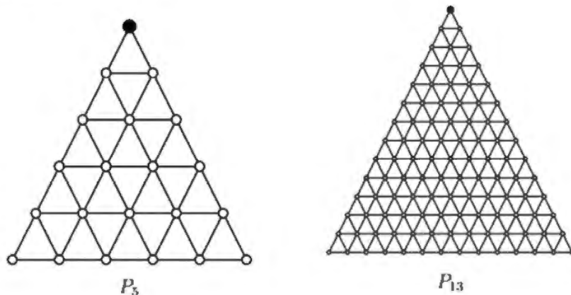
Figure 1: Pyramids P_5 and P_{13}
