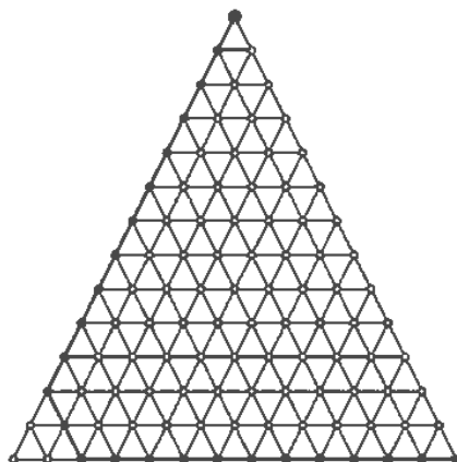
Figure 3: A game progression in which forts arise
