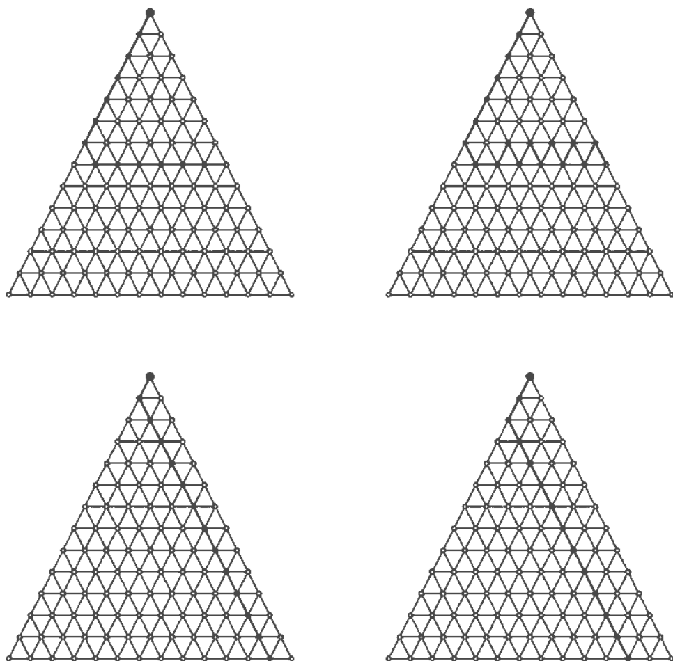
Figure 2: Game progressions in which no forts arise
