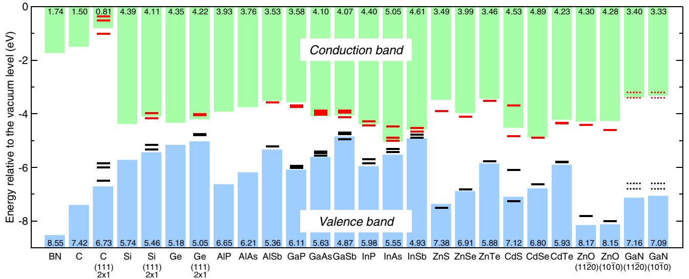
FIG. 2. (Color online) Band alignment based on the ionization potential (IP) and electron affinity (EA) obtained using GW\Gamma^1 @HSE. The surface orientation is (110) unless otherwise noted. Experimental values reported for the corresponding surfaces are indicated by solid horizontal bars except for GaN, for which values for polar {0001} surfaces are shown with broken bars [77,78]. The theoretical IP and EA values are shown as numbers at the bottom and top of the figure, respectively. Note that the IP and EA correspond to the negatives of the valence band maximum and conduction band minimum with respect to the vacuum level, respectively.
