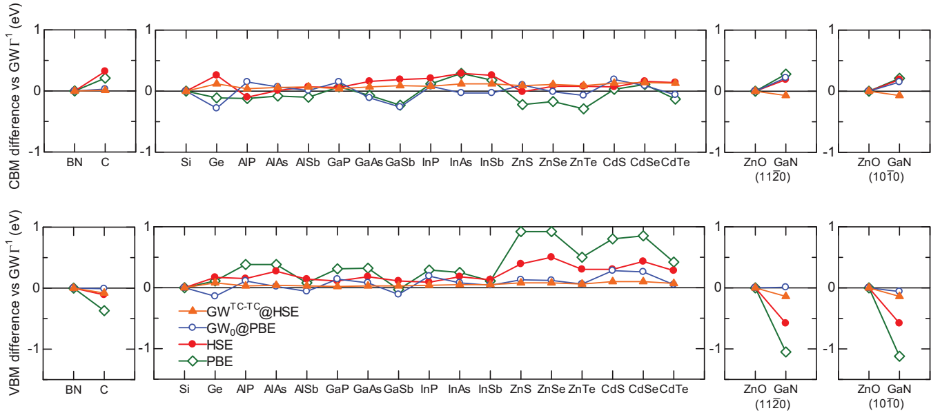
FIG. 5. (Color online) Deviations in the valence band maximum (VBM) and conduction band minimum (CBM) from GW\Gamma^1 @HSE for PBE, HSE, GW_0 @PBE, and GW^{TC-TC} @HSE in the interfacial offset-based alignment. The values are relative to those for BN, Si, and ZnO in the respective panels.
