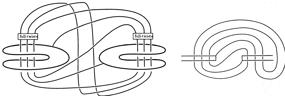
Figure 3.2: K(7, 4|2, 2)
