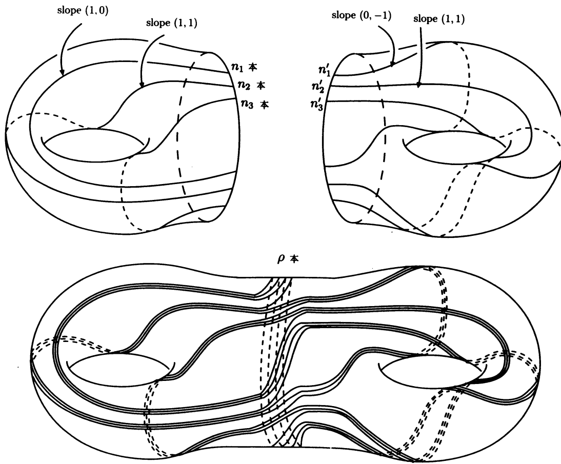
Figure 2.1: K\{(3, 3, 3; 3, 3, 3|4)(1, 0, 1, 1)(0, -1, 1, 1)\}
