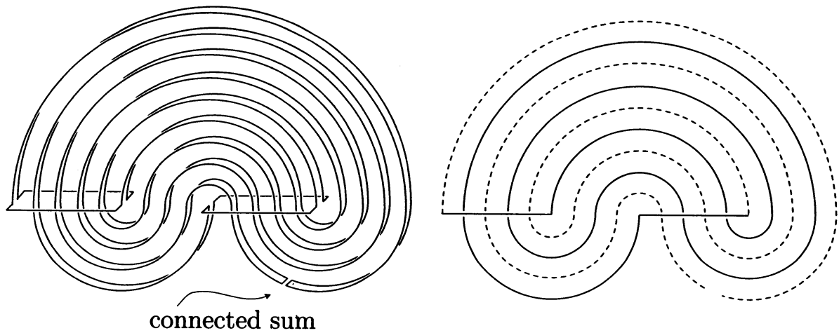
Figure 3.3: The connected sum of B(5,4) and -B(5,4) .
