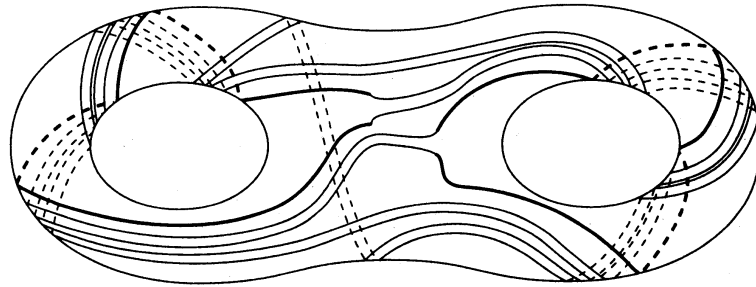
K(5, 2|2, 2)
