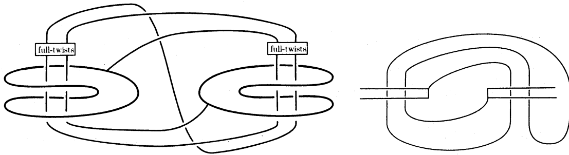
Figure 3.1: K(5, 2|2, 2)
