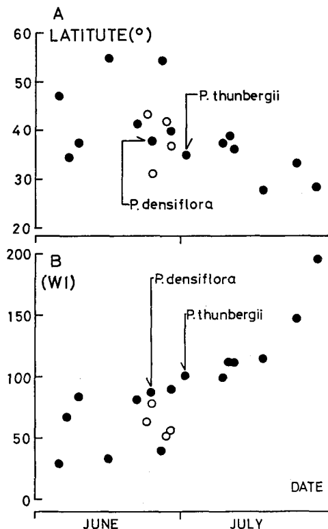
Fig. 3. Relation between completion date of cones and mean latitude of native region in each pine species (A), and relation between completion date and values of WI (B). Open circle: Haploxylon pines. Solid circle: Diploxylon pines.
