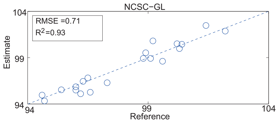
Figure 11: API content estimation result by NCSC-GL
