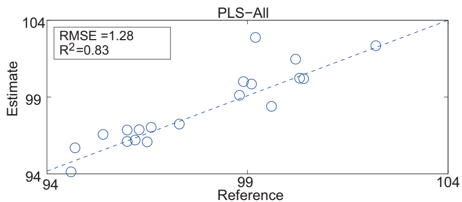
Figure 3: API content estimation result by PLS-All
