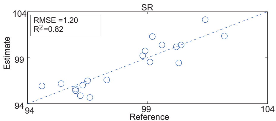
Figure 6: API content estimation result by SR
