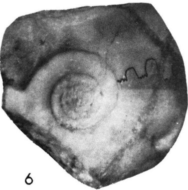
NAKAZAWA and BANDO, Triassic Ammonites from Timor
