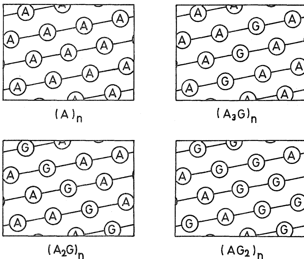
Fig. 7. Radial projections showing distributions of L-alanyl (A) and glycyl (G) residues on \alpha -helices of sequential polypeptides.
