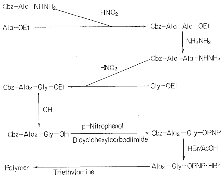
Fig. 1. Synthetic steps of sequential polypeptide, (\text{A}_2\text{G})_n .
