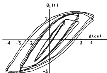
(a) Shear Force in Column ①.
