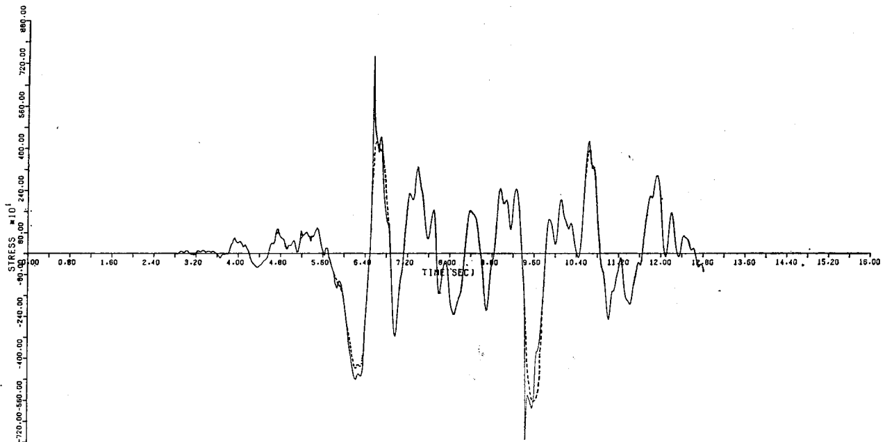
Fig. 12 Stress response.
