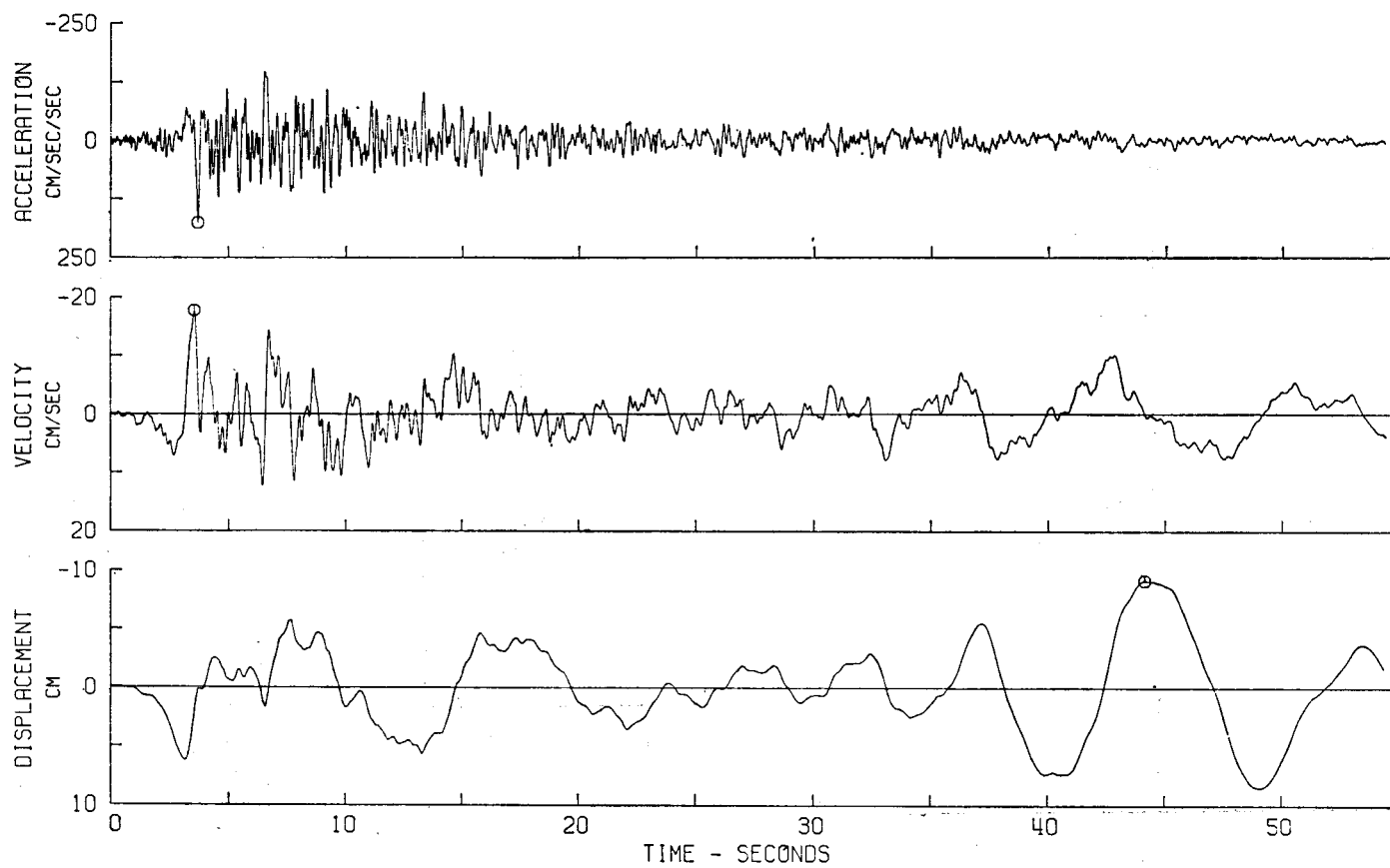
Fig. 9 S69E component of accelerogram at Taft during the 1952 Kern Country, California Earthquake.
