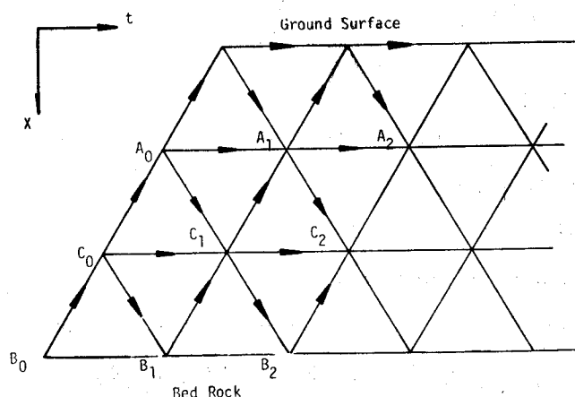
Fig. 4 Characteristics net.
