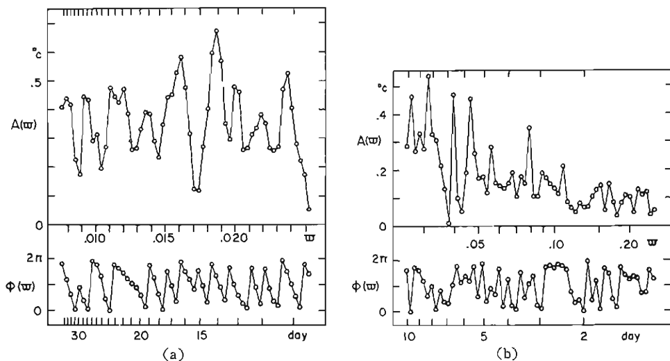
Fig. 4. Spectral amplitude and phase of the temperature at the Wakayama Meteorological Observatory.
