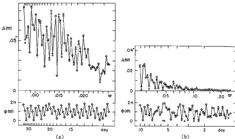
Fig. 1. Spectral amplitude A(\omega) and phase \phi(\omega) of the E-W component tilt observed at Akibasan. The cross represents the corrected values for oceanic tides, temperature, atmospheric pressure and its time gradient.
