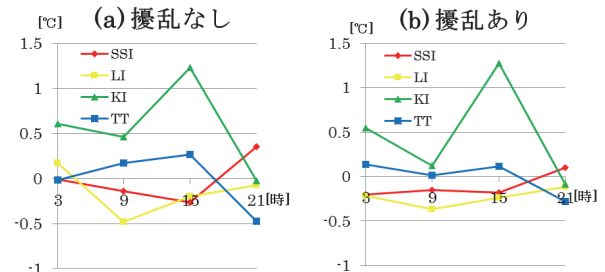
Fig. 20 The differences of stability indices between the Kii mountains and the Chugoku mountains for (a) the undisturbed and (b) the disturbed cases.
