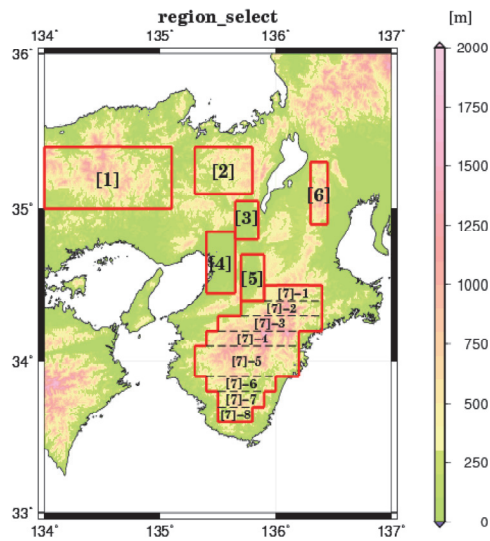
Fig. 12 The divided areas within the analysis region.
