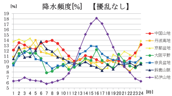
Fig. 13 The diurnal variation of the area-averaged frequency of precipitation under undisturbed conditions.
