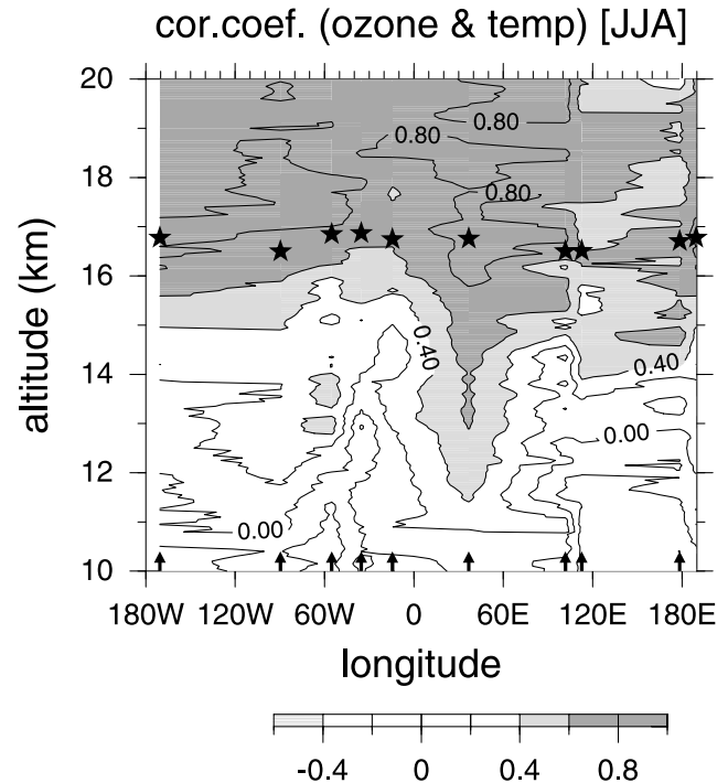
Figure 8. Longitude-altitude section of the correlation coefficient between the ozone mixing ratio and the temperature in JJA.
