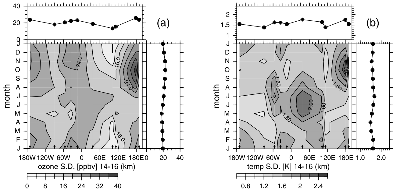
Figure 7. As Figure 5, but for contour plots of (a) the ozone standard deviation (ppbv) and (b) the temperature standard deviation (K) averaged over 14–16 km.
