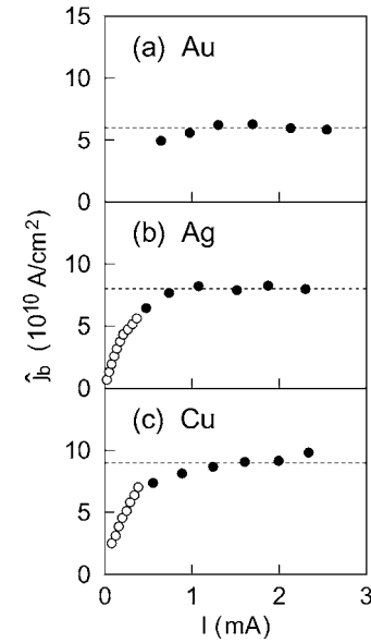
FIG. 4. Current density \hat{j}_b at contact break estimated from \hat{G}_b for (a) Au, (b) Ag, and (c) Cu. Filled and empty circles represent \hat{j}_b 's corresponding to \hat{G}_b 's shown by gray lines in Figs. 3 and 5, respectively. A dashed line in each plot indicates a critical current density j_c for the current-induced contact break.
