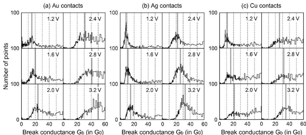
FIG. 3. Break conductance histograms of noble metal contacts obtained at V_a \geq 1.2 V. Each histogram shows a broad peak structure, the position of which is indicated by a gray line.
