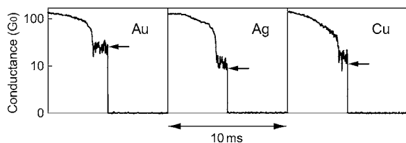
FIG. 2. Examples of transient conductance trace recorded on Au, Ag, and Cu contacts at V_a = 2.4 V. The conductance scale is strongly nonlinear reflecting the nonlinear signal-to-conductance conversion in our measurements. In each trace, the conductance shows appreciable fluctuation before the contact breaks off. Arrows indicate locations of the break conductance G_b .
