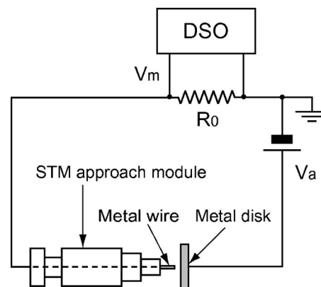
FIG. 1. Schematic of our experimental setup. A contact is made and broken repeatedly between a metal wire and a disk by oscillating the wire against the disk using a tubular PZT scanner. Transient conductance upon contact break is recorded by a fast digital storage oscilloscope (DSO), which monitors voltage drop across a current-sensing resistor R_0 connected in series with the contact.
