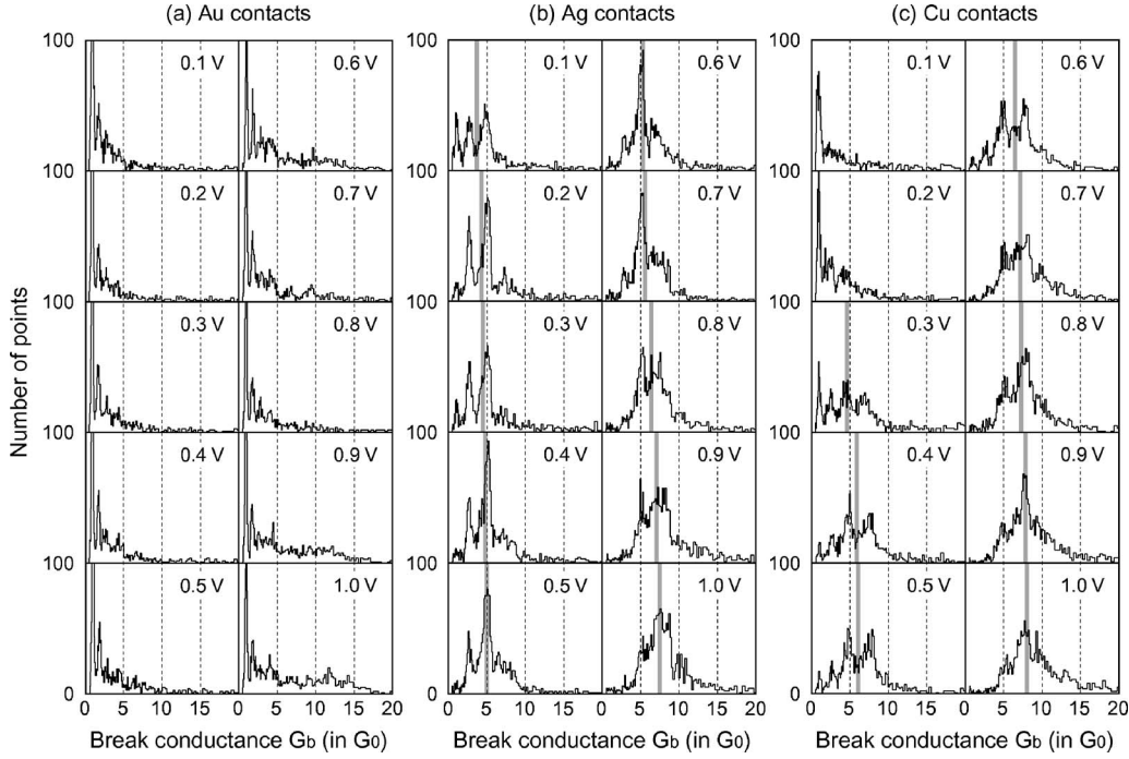
FIG. 5. Break conductance histograms of noble metal contacts obtained at V_a \leq 1.0 V. Histograms show a couple of sharp peaks corresponding to certain stable contact geometries. Gray strip lines indicate values of \hat{G}_b of the current-induced break, which weakly influences the break of Ag and Cu contacts as explained in the text.
