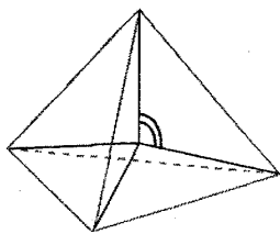
Figure 1: \theta = \cos^{-1}(-\frac{1}{3})
