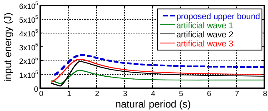
Fig.5 Proposed upper bound of earthquake input energy and realized earthquake input energy for three earthquake ground motions
