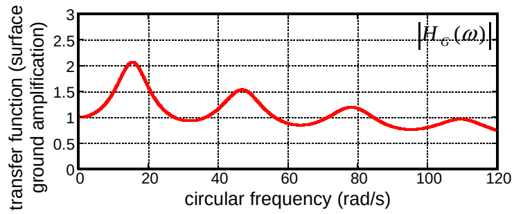
Fig.10 Transfer function of shallow ground of nominal model
