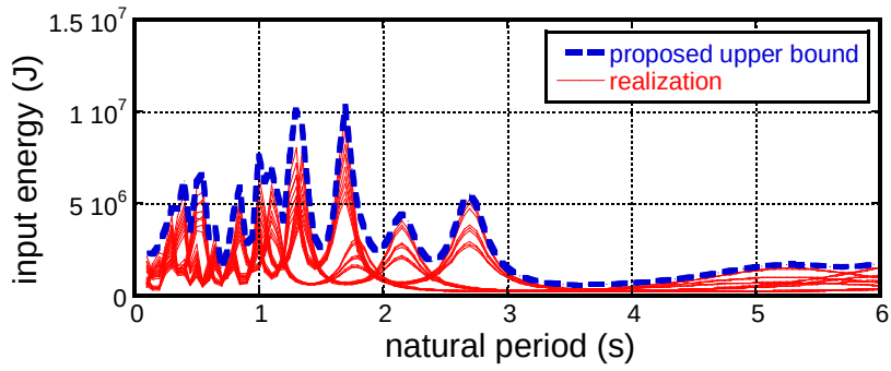
Fig.16 Proposed upper bound of earthquake input energy to SR model on uncertain shallow and deep ground subjected to certain input at earthquake bedrock
