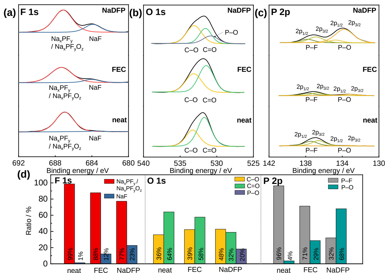
Fig. 7 X-ray photoelectron spectra of the SEI layers formed on the HC electrodes after 20 cycles in 1 M \text{NaPF}_6 -EC/DMC (1:1, v:v) electrolyte with 0 wt% NaDFP (neat), 1 wt% NaDFP and 3 wt% FEC additives in the (a) F 1s, (b) O 1s, and (c) P 2p regions, and (d) SEI component ratios (see Table S8 in ESI† for the binding energy of the peaks).
