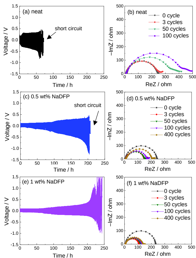
Fig. 2 Voltage profiles and Nyquist plots of the Na/Na symmetrical cells during galvanostatic Na metal deposition/dissolution cycles using 1 M \text{NaPF}_6\text{-EC/DMC} (1:1, v:v) electrolyte with (a, b) 0 wt% NaDFP (neat), (c, d) 0.5 wt% NaDFP and (e, f) 1 wt% NaDFP. Current density: 1 \text{ mA cm}^{-2} . (See Fig. S6 in ESI† for voltage profiles and Nyquist plots with 0.5 wt% FEC and 3 wt% FEC)
