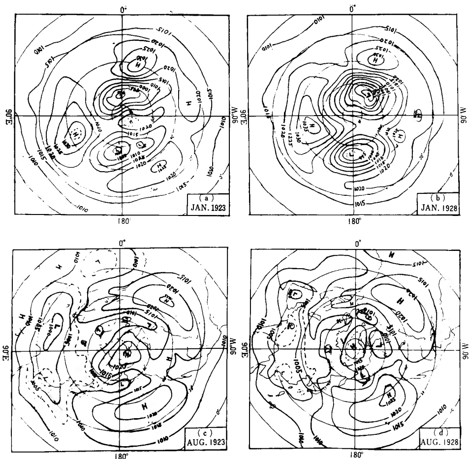
Fig. 4. Monthly mean weather plotting chart at sea level (after U. S. W. B). (a)—Jan. 1923 (b)—Jan. 1928 (c)—Aug. 1923 (d)—Aug. 1928
