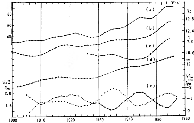
Fig. 7. Secular trend of sunspot number, annual mean atmospheric and water temperature, sea level and zonal and meridonal component of winter mean atmospheric pressure gradient near Japan.
