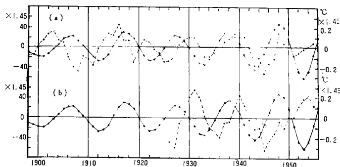
Fig. 5. Comparison between sunspot number and annual mean atmospheric temperature (5 stations' mean in Japan) and annual mean water temperature (4 stations' mean in Japanese waters).
