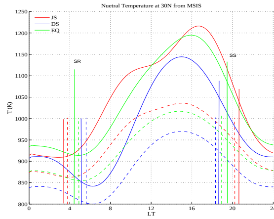
Figure 3. Diurnal variation of the neutral temperature at 30N geographic latitude in various seasons calculated from MSISE90 model. Solid lines are for 400 km altitude, and the dashed ones for 200 km altitude. Vertical lines denote corresponding time for sunrise and sunset. Note that at both heights, the temperature variation is sharper at dusk than at dawn.
