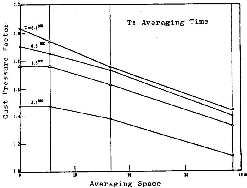
Fig. 6 Variations of gust pressure factors with averaging space and time. ( T ; averaging time of velocity pressure).
