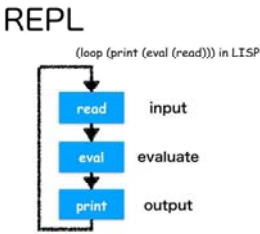
図 3: read, evaluate, print loop (REPL).
