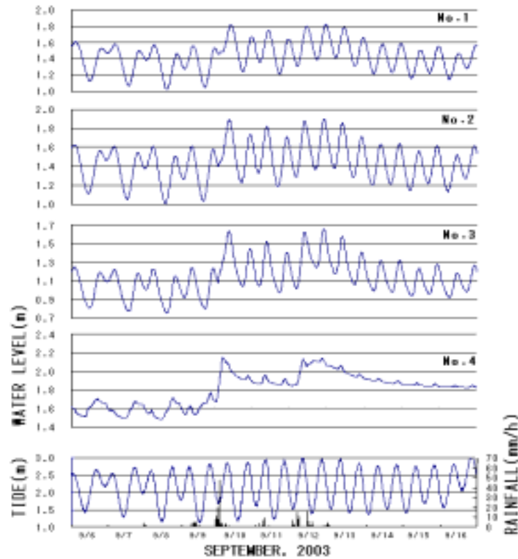
Fig. 4 Water level changes at Saga. From the top, raw data of water levels, ocean tide level and rainfall from September 06 to September 16, 2003.
