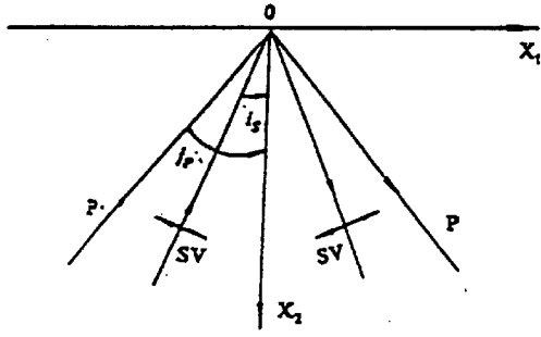
Fig. 1 P-, SV-wave system incident upon free ground surface
