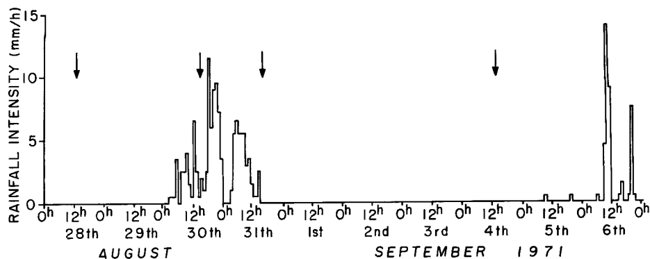
Fig. 11 The hyetograph corresponding to Fig. 10. The timing of the observation of soil moisture is shown with arrows.
