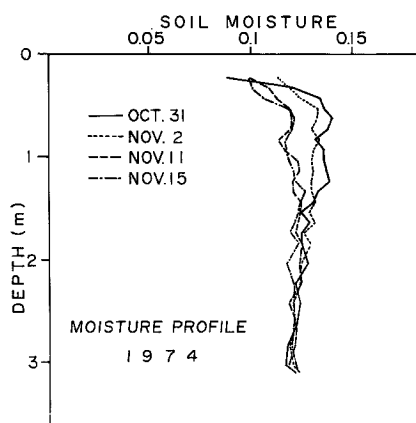
Fig. 8 Time change in the soil moisture profile during the period corresponding to Figs. 6 and 7 at the same location.
