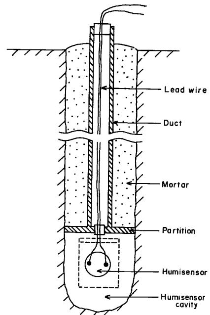
Fig. 4 A schematic illustration of the installation of humisensor (an electrical hygrometer element) in a bore-hole. Several humisensors are installed at different depths.
