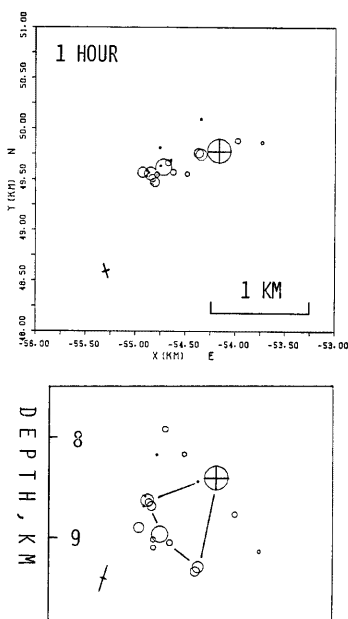
Fig. 7 Same as Fig. 6, but during only one hour after the occurrence of the largest aftershock. The inferred fault plane of the largest aftershock is represented by a triangular area in the cross section. Crossed bars indicate the error extent of hypocenters caused by 10 msec reading error of P-wave arrival times at five stations.
