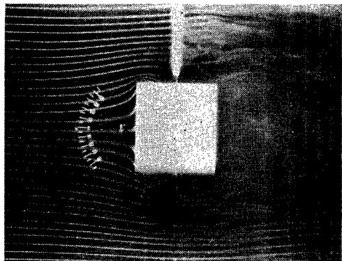
Photo. 14 The stream line around the moving square cylinder.
