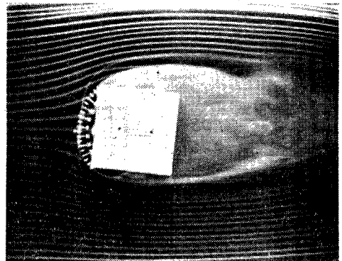
Photo. 4 The stream line around the square cylinder for angle of attack 5^\circ .
