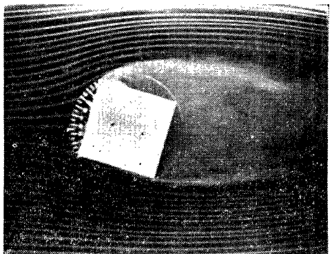
Photo. 6 The stream line around the square cylinder for angle of attack 15^\circ .
