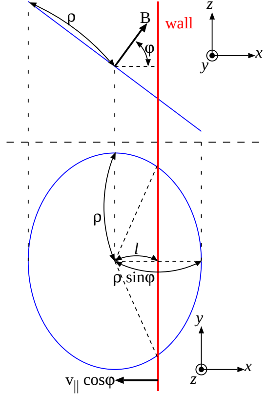
Figure 4.7: Schematic diagrams of a particle trajectory on the gyrocenter frame. The particle motion is simple gyration and the wall is approaching from the right hand side with the velocity v_{||} \cos \varphi .
