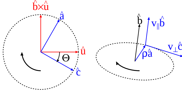
Figure 2.2: Definition of the gyrophase. An unit vector \hat{\mathbf{u}} is used as the base direction.
