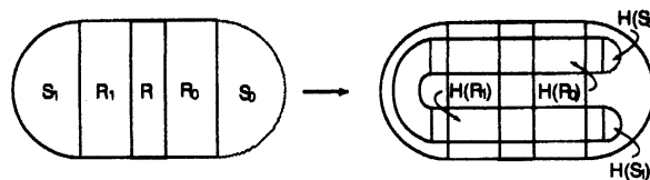
Figure 3: Smale-horseshoe map
