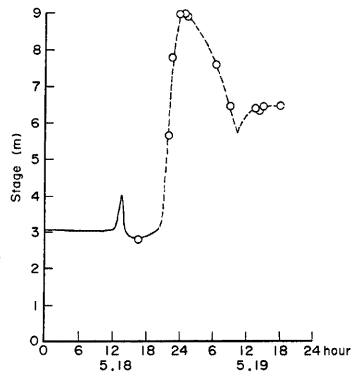
Fig. 15 Water Stage variation at Dastle Rock.
