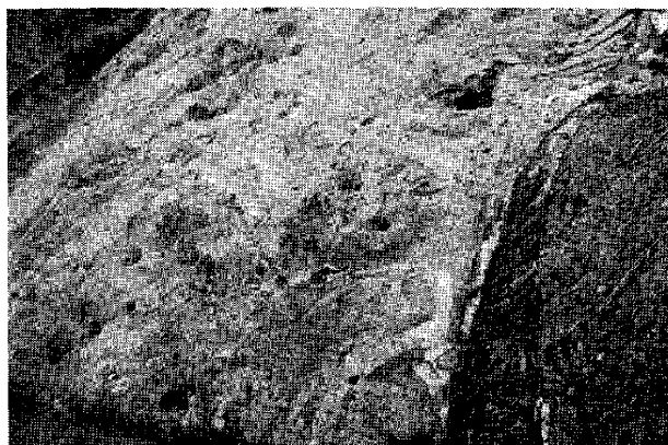
Photo. 10 The depression holes on the debris avalanche deposit.
