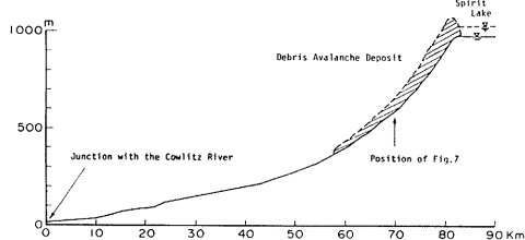
Fig. 6 Longitudinal profile of the debris avalanche deposit along the North Fork Toutle River.
