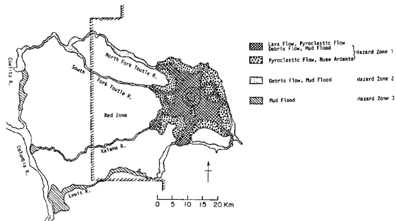
Fig. 19 Hazard map due to the eruption of Mt. St. Helens after Crandell and Mullinaux 11) .
