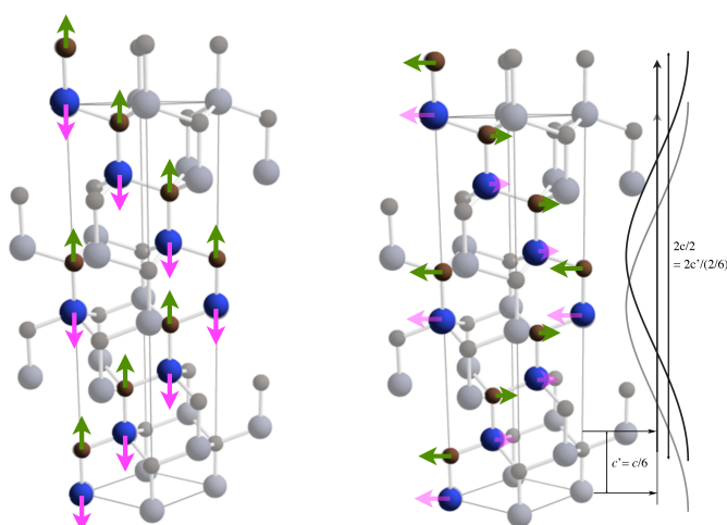
FIG. 2 A_1 mode ( 970\text{ cm}^{-1} , FLO(0); left) and E_2 mode ( 790\text{ cm}^{-1} , FTO(2/6); right).
