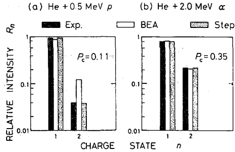
Fig. 8. Observed and calculated relative intensities of ionized helium atoms excited by protons and alpha particles against the charge state. (a) by 0.5 MeV protons, (b) by 2.0 MeV alpha particles.
