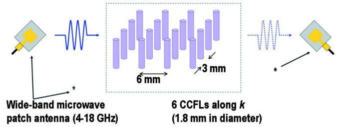
FIG. 6. (Color online) Experimental schematic setup for wave transmittance.
