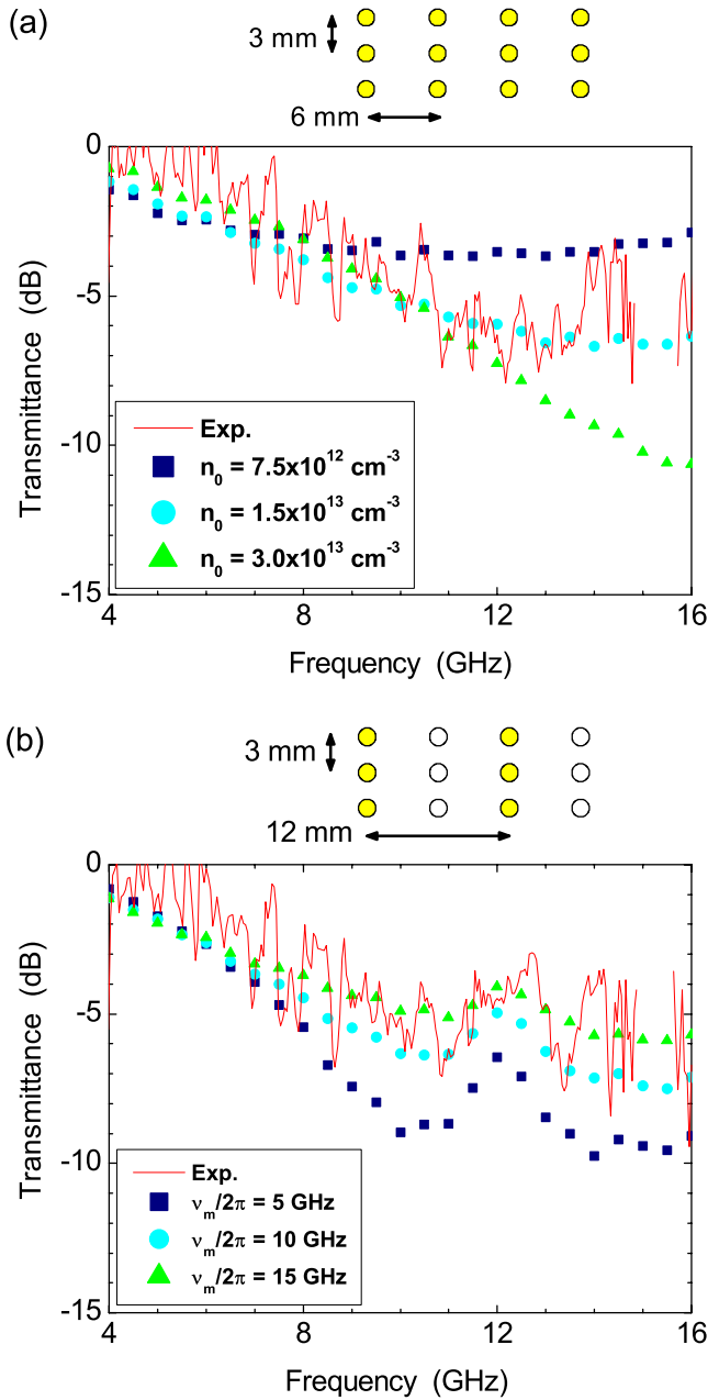
FIG. 7. (Color online) Experimental data of transmittance in TE mode (a) in 6 mm periodicity and (b) in 12 mm. The dots indicate numerical results and we set n_e in the center of the column = 1.5 \times 10^{13} \text{ cm}^{-3} and \nu_m/2\pi = 12.5 \text{ GHz} if there are no specific notes.
