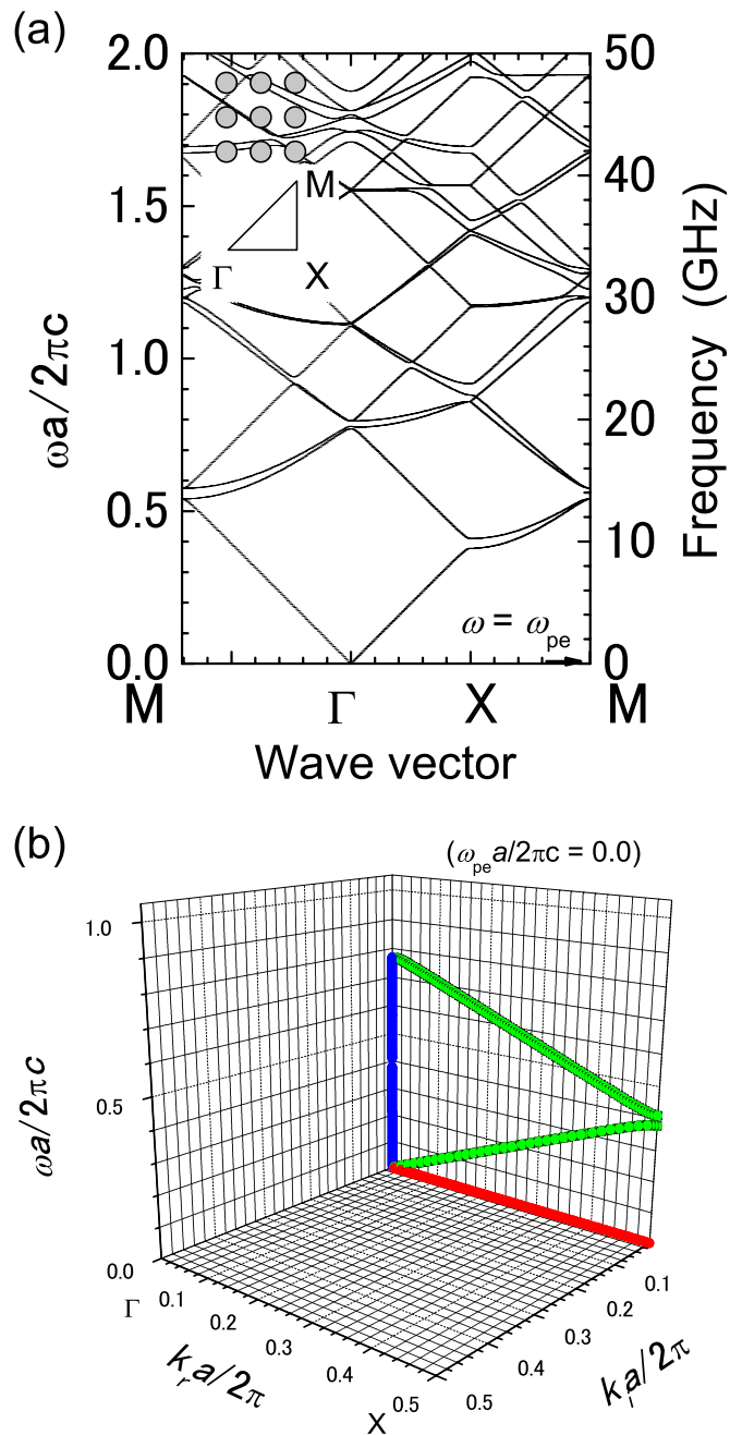
FIG. 3. (Color online) Dispersion relation derived using plane-wave expansion method in TE mode in a square lattice of 12 mm with filling factor of 0.18. Vacuum holes are surrounded by dielectric with \epsilon=1.8 , and there is no plasma. (a) Photonic band of k_r . (b) Branch around lowest photonic band gap in the \Gamma -X direction in 3D space.
