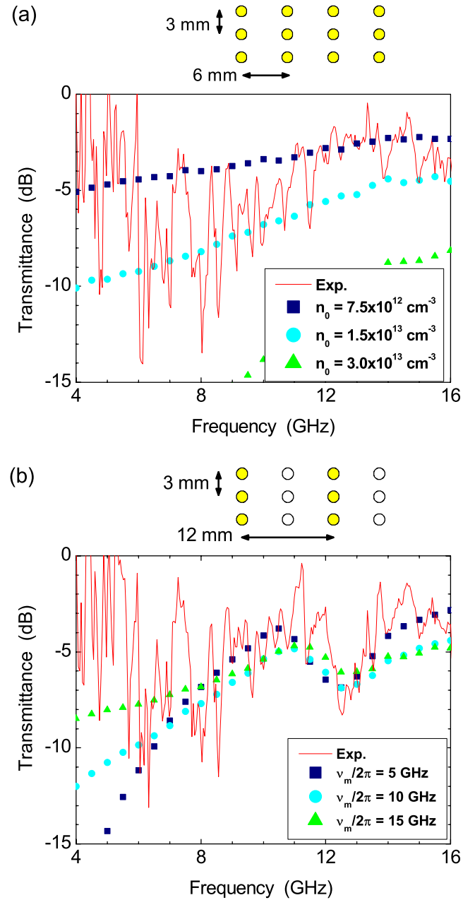
FIG. 8. (Color online) Experimental data of transmittance in TM mode (a) in 6 mm periodicity and (b) in 12 mm. The dots indicate numerical results and we set n_e in the center of the column = 1.5 \times 10^{13} \text{ cm}^{-3} and \nu_m/2\pi = 12.5 \text{ GHz} if there are no specific notes.
