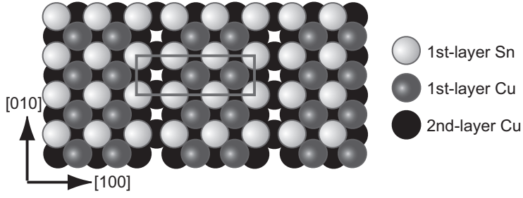
Fig. 9. Top view of the structure model for Cu(001)- (3\sqrt{2} \times \sqrt{2})R45^\circ -Sn [75]. Rectangle shows the unit cell.
