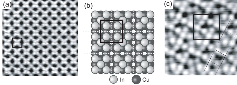
Fig. 8. (a) STM image for the (2\sqrt{2} \times 2\sqrt{2})R45^\circ surface. (b) Line-dislocation model for (2\sqrt{2} \times 2\sqrt{2})R45^\circ . Solid lines indicate the unit cell. White broken lines indicate the line vacancies formed in the (1 \times 1) lattice of In. Note that the actual In atom positions are shifted from four-fold hollow sites. (c) STM image for the (\sqrt{20} \times \sqrt{20})R26.6^\circ surface [70]. Solid lines indicate the unit cells. The dotted lines indicate the (2 \times 2) mesh.
