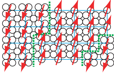
Fig. 17. A possible Ising-model representation of the order-disorder ((2\sqrt{2} \times 2\sqrt{2})R45^\circ - (2 \times 2)) transition on In/Cu(001). Overlaid square lattice is for (2\sqrt{2} \times 2\sqrt{2})R45^\circ . Broken lines indicate anti-phase boundary.
